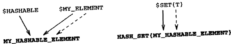
Fig. 1. Typical inheritance graph for $HASHABLE
