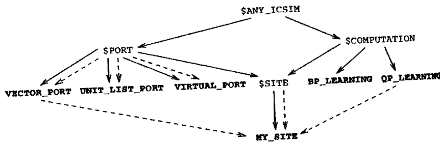
Fig. 2. Multiple Subclassing for Programming by Configuration
